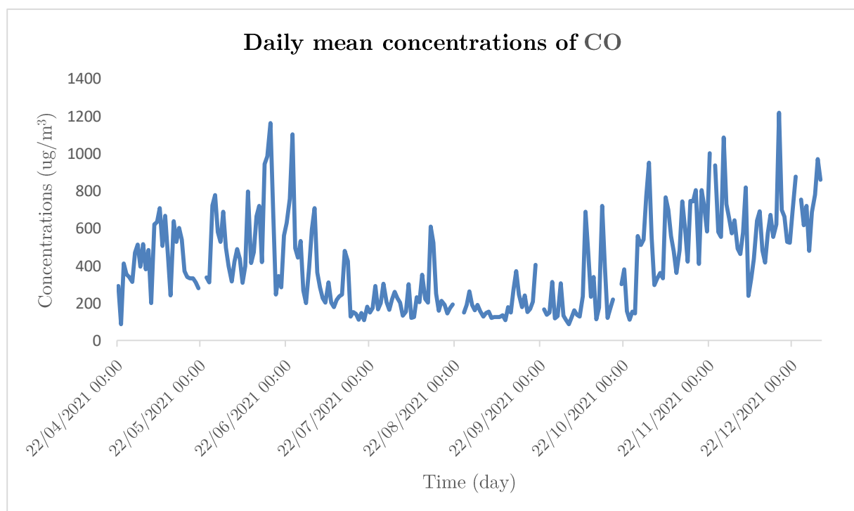
Fig. 6. Daily variations in CO concentrations (µg/m 3 ) in ambient air at the Attécoubé lagoon, from April to December 2021.
