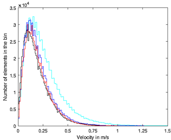
Fig. 7. Same as Fig. 6 but for FADs.
