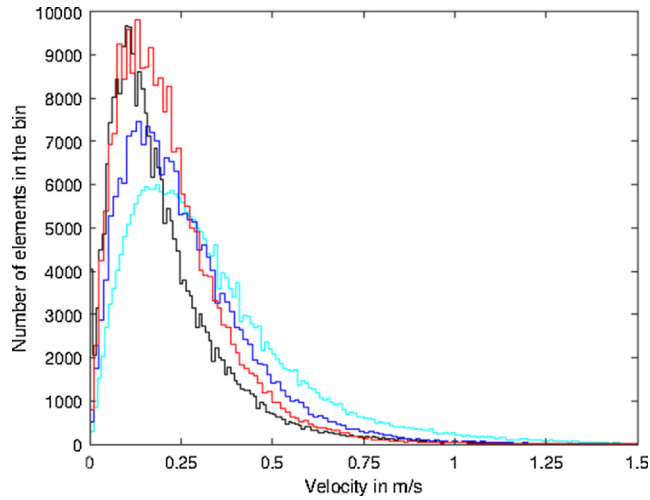
Fig. 6. Velocity distributions of (cyan) observed drifters and simulated particles obtained with (black) CROCO, (red) OSCAR and (blue) GlobCurrent in the Tropical Atlantic. (For interpretation of the references to colour in this figure legend, the reader is referred to the web version of this article.)
