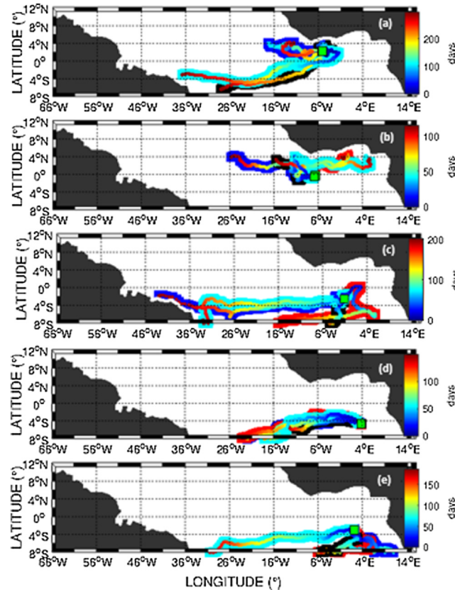
Fig. A.4. Same as Fig. 3 for (a) FAD 9740, (b) FAD 379, (c) FAD 14865, (d) FAD 731 and (e) FAD 14890.
