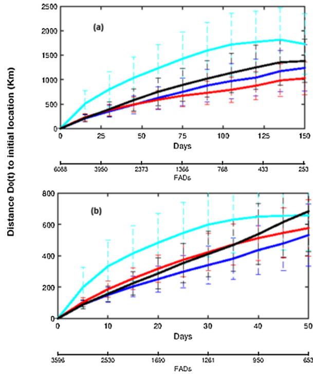
Fig. A.12. Same as Fig. A.11 but for FADs.
