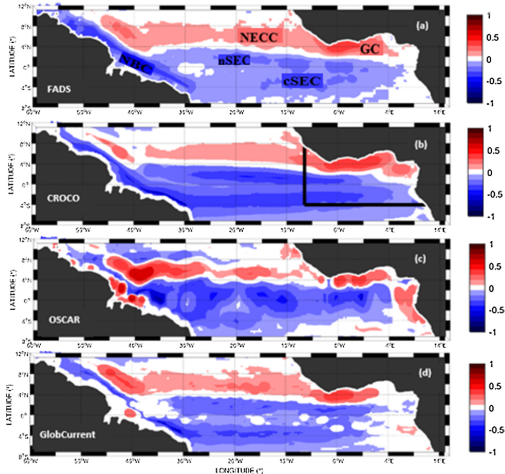
Fig. A.1. Same as Fig. 2 but the mean annual zonal velocity covers the period of FAD data.
