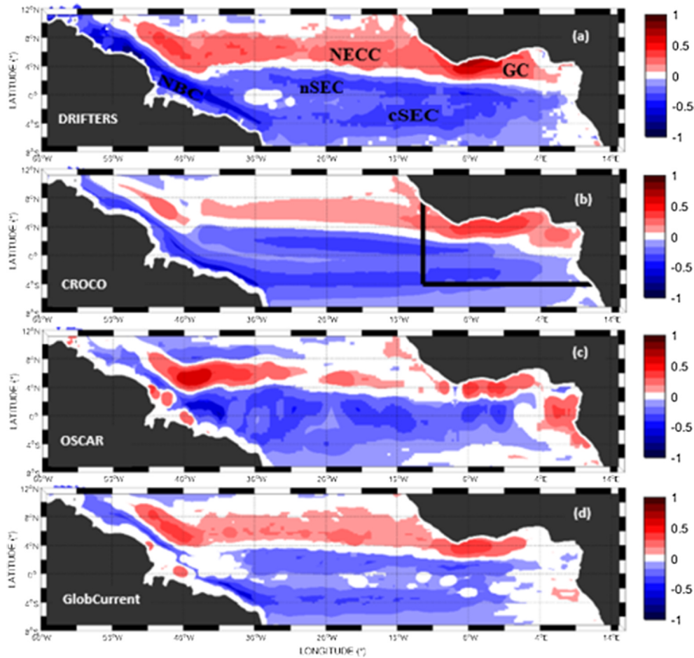
Fig. 2. Mean annual zonal velocity ( \text{m s}^{-1} ) over the period 1997–2014 for (a) NOAA's drifters, (b) CROCO model, (c) OSCAR and (d) GlobCurrent in the Tropical Atlantic. The North Brazil Current (NBC), north and central branches of the South Equatorial Current (nSEC and cSEC), the North Equatorial Counter Current (NECC) and the Guinea Current (GC) are indicated in (a). Solid lines in (b) indicate the boundaries of the Gulf of Guinea. The cell size in (a) is 1^\circ \times 1^\circ and the number of drifters in each cell is shown in Fig. 4a.
