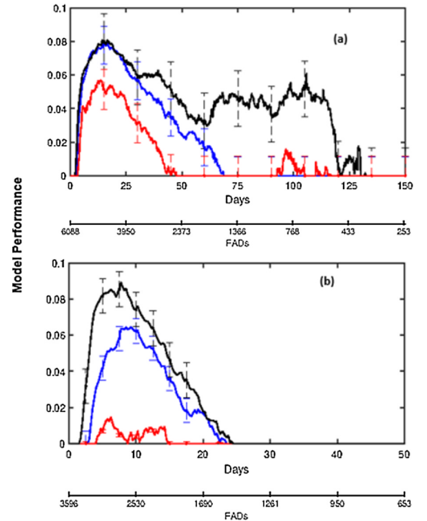
Fig. 9. Same as Fig. 8 but for FADs.
