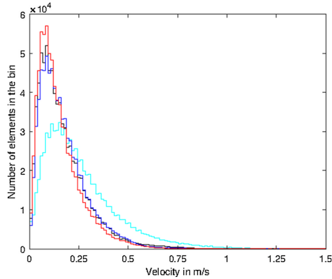
Fig. A.22. Same as Fig. 7 but using the barycenter of a cloud of 1,000 particles released at the observed FAD initial locations.
