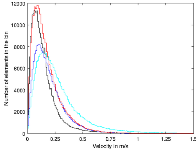
Fig. A.7. Same as Fig. 6 but the distributions of velocity fluctuations are represented for drifters.
