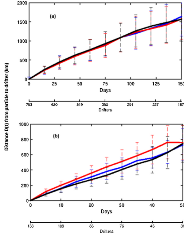
Fig. A.9. Mean separation distance (or model error distance) over time between simulated particles and NOAA drifters obtained with (black) CROCO, (red) OSCAR and (blue) GlobCurrent for (a) the whole Tropical Atlantic and (b) the Gulf of Guinea. (For interpretation of the references to colour in this figure legend, the reader is referred to the web version of this article.)
