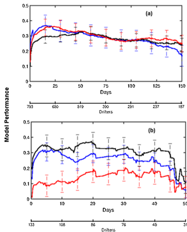
Fig. A.20. Same as Fig. A.19 but using the barycenter of a cloud of 1,000 particles released around (radius R = 50 km) observed drifters initial locations.
