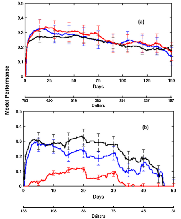
Fig. 8. Mean model performance or skill obtained with (black) CROCO, (red) OSCAR, and (blue) GlobCurrent, (a) for the Tropical Atlantic and (b) the Gulf of Guinea. Note that the number of drifters used for the mean skill calculation (lower scale) decreases with time and that the time periods represented in the two panels are different. The vertical bars represent the standard deviation. (For interpretation of the references to colour in this figure legend, the reader is referred to the web version of this article.)
