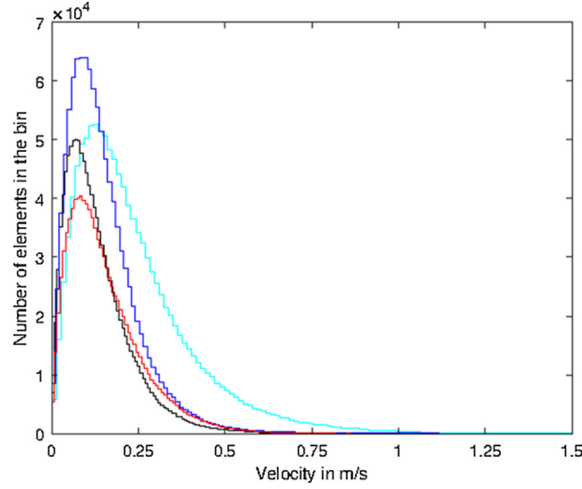
Fig. A.8. Same as Fig. A.7 but for FADs.
