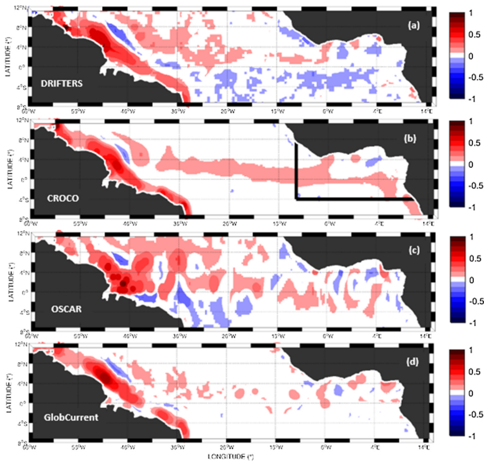
Fig. A.2. Same as Fig. 2 but the mean annual meridional velocity is represented.
