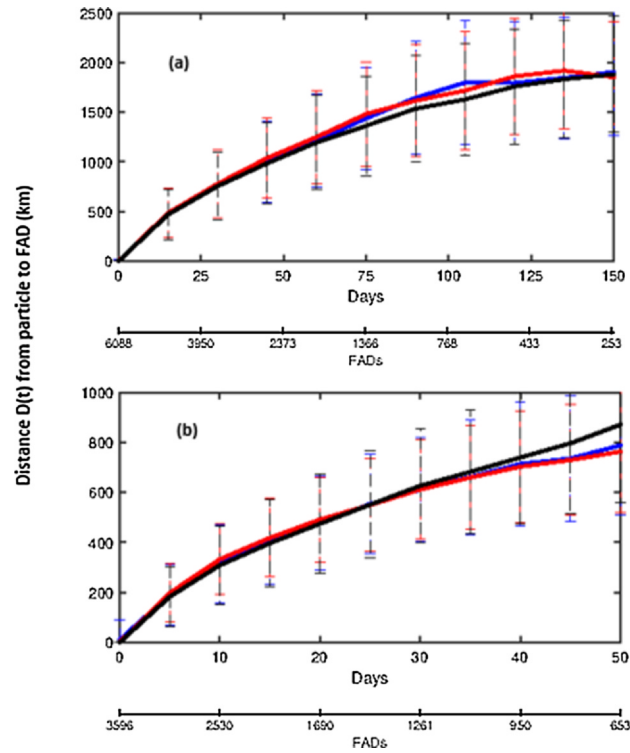
Fig. A.10. Same as Fig. A.9 but for FADs.
