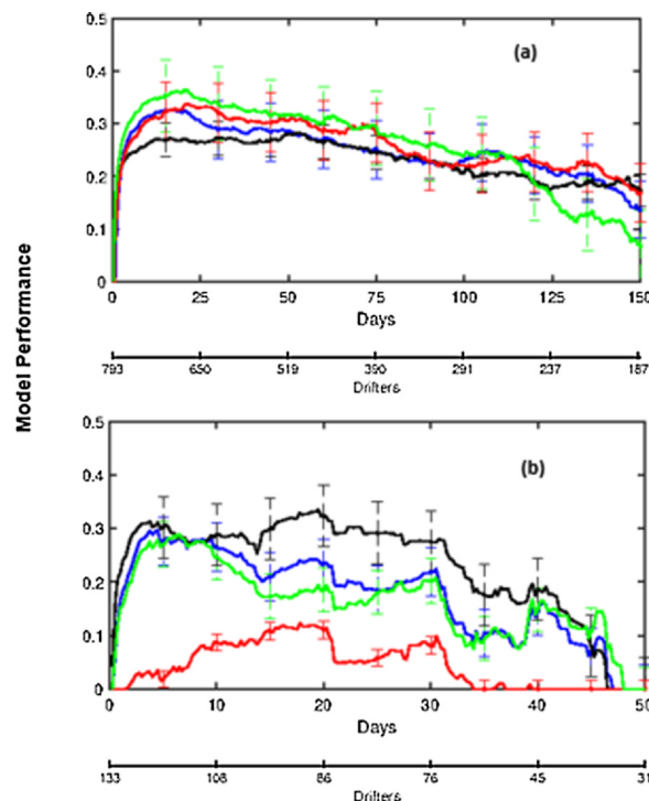
Fig. A.17. Same as Fig. 8 but with 3-h output currents (green) as opposed to 1-day (blue) for GlobCurrent. (For interpretation of the references to colour in this figure legend, the reader is referred to the web version of this article.)
