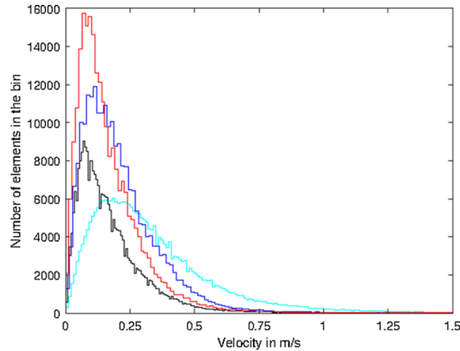
Fig. A.18. Same as Fig. 6 but using the barycenter of a cloud of 1,000 particles released at the observed drifters initial locations.
