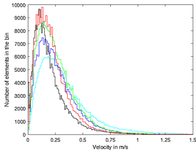
Fig. A.16. Same as Fig. 6 but with 3-h output currents (green) as opposed to 1-day (blue) for GlobCurrent. (For interpretation of the references to colour in this figure legend, the reader is referred to the web version of this article.)
