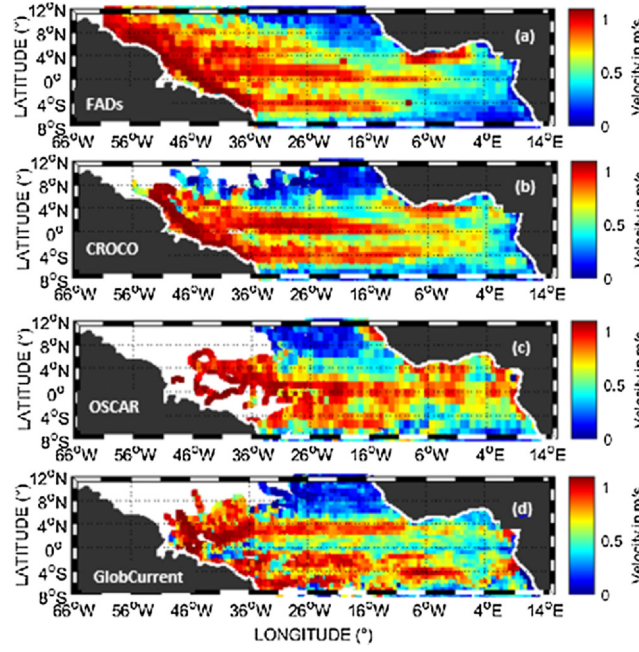
Fig. A.6. Same as Fig. A.5 but for FADs.
