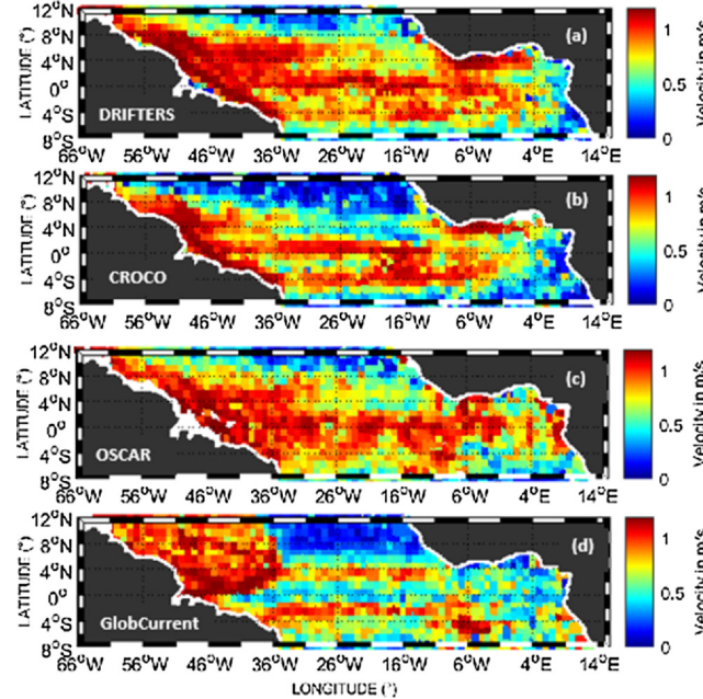
Fig. A.5. Mean velocity of (a) drifters and simulated particles (using (b) CROCO, (c) OSCAR and (d) GlobCurrent) passing through grid cells of 1^\circ \times 1^\circ . Grid cells with zero drifters or simulated particles are shown in white.
