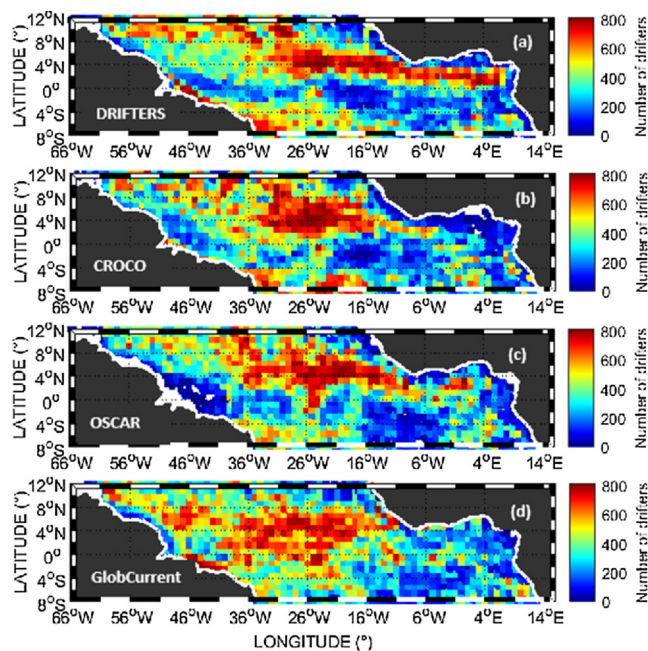
Fig. 4. Densities of (a) observed drifters and simulated particles (using (b) CROCO, (c) OSCAR and (d) GlobCurrent) computed as the average of the number of drifters or simulated particles passing through grid cells of 1^\circ \times 1^\circ . Grid cells with zero drifters or simulated particles are shown in white.
