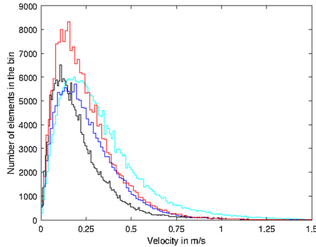
Fig. A.13. Same as Fig. 6 but when particles are reset every 10 days at the observed drifters locations.
