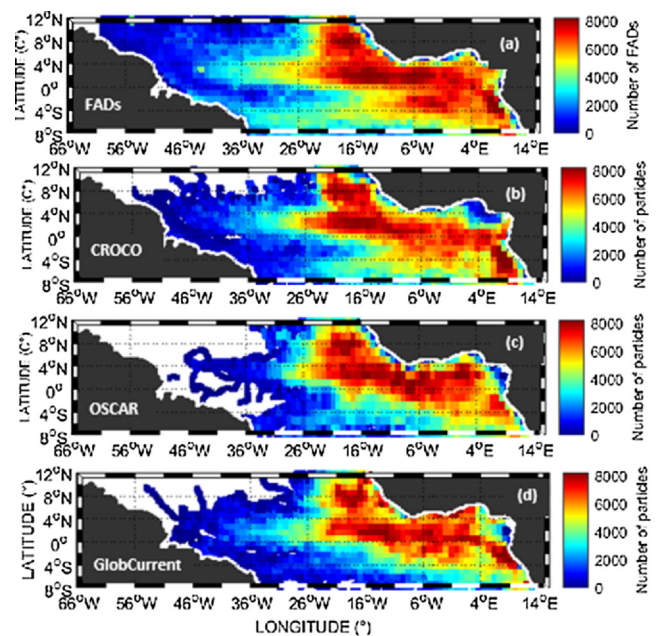
Fig. 5. Same as Fig. 4 but for FADs.
