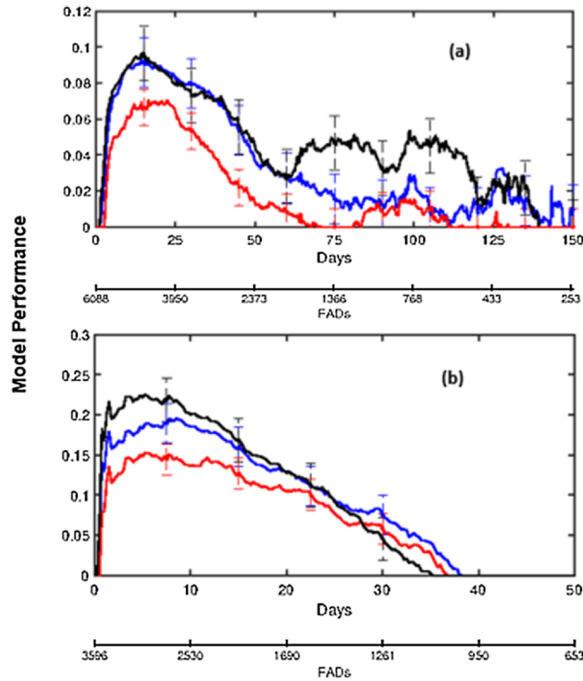
Fig. A.23. Same as Fig. 9 but using the barycenter of a cloud of 1,000 particles released at the observed FAD initial locations.
