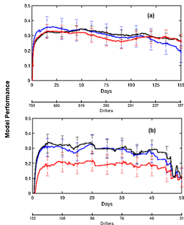
Fig. A.21. Same as Fig. A.20 but with R = 200 km.
