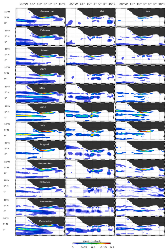
Fig. A.24. Monthly climatology of Eddy Kinetic Energy (EKE, \text{m}^2/\text{s}^2 ) over the Gulf of Guinea: (a) for CROCO, (b) for OSCAR and (c) for GlobCurrent.
