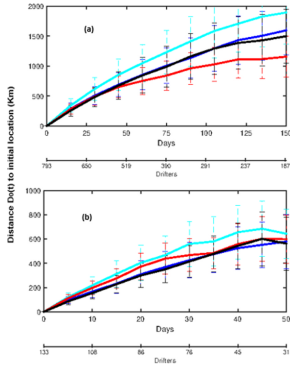
Fig. A.11. Mean absolute dispersion (or distance to release location) over time obtained for (cyan) NOAA drifters and simulated particles with (black) CROCO, (red) OSCAR and (blue) GlobCurrent for (a) the whole Tropical Atlantic and (b) the Gulf of Guinea. (For interpretation of the references to colour in this figure legend, the reader is referred to the web version of this article.)
