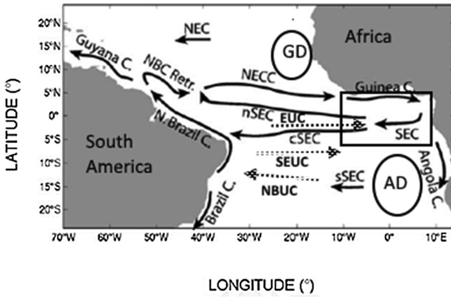
Fig. 1. Schematic of oceanic circulation, the major surface (respectively, subsurface) currents are represented in arrows in solid lines (respectively, dashed lines): North Equatorial CounterCurrent (NECC), Guinea Current (GC), Equatorial UnderCurrent (EUC), Angola Current (AC), northern (nSEC), central (cSEC) and southern (sSEC) branches of the South Equatorial Current (SEC), South Equatorial UnderCurrent (SEUC), North Brazil Currents (NBC) and its retroflection (NBC retr.), North Brazil UnderCurrent (NBUC), Brazil Current (BC) and Guyana Current (GC). Rectangle and ellipses represent respectively the Gulf of Guinea region, Guinea Dome (GD) and Angola Dome (AD) (adapted from Lumpkin and Garzoli (2005)).
