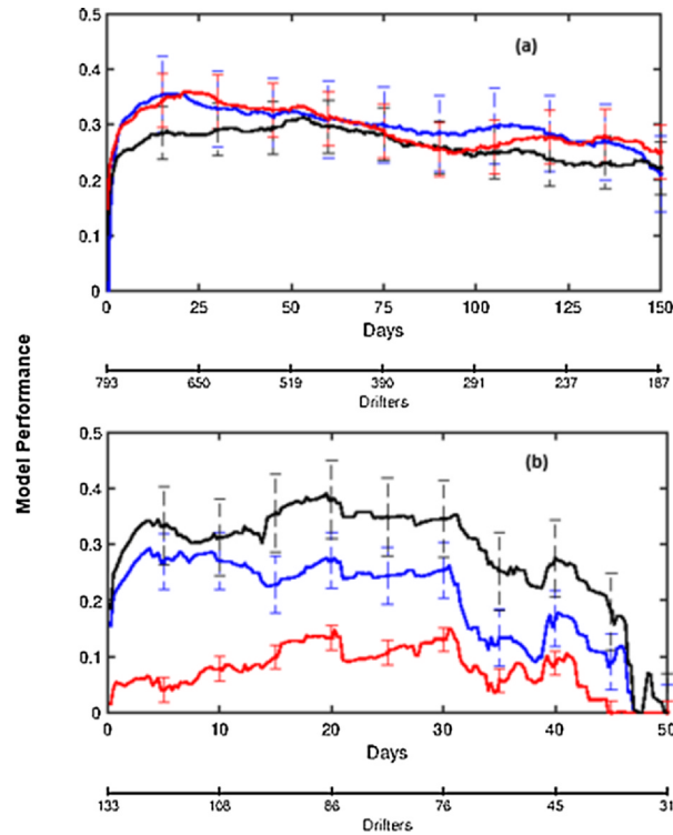
Fig. A.19. Same as Fig. 8 but using the barycenter of a cloud of 1,000 particles released at the observed drifters initial locations.
