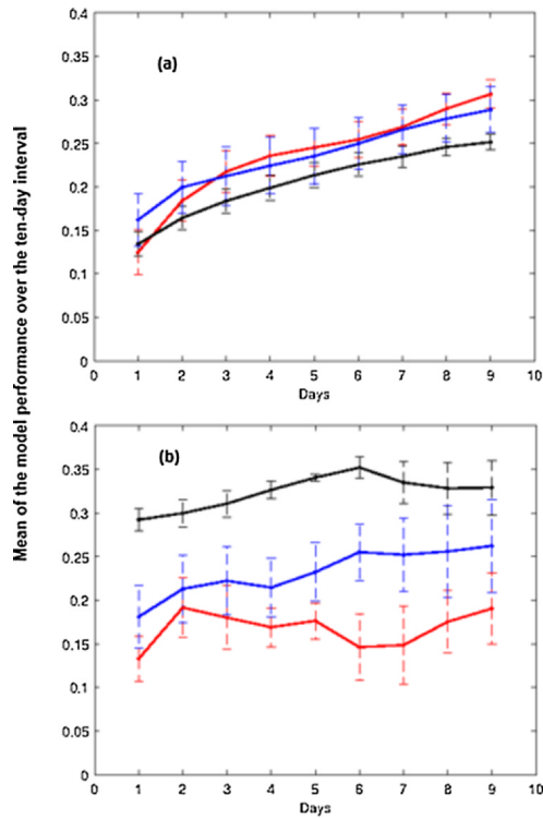
Fig. 10. Mean of the model performance over the ten-day interval when particles are reset every 10 days at the observed drifters locations.
